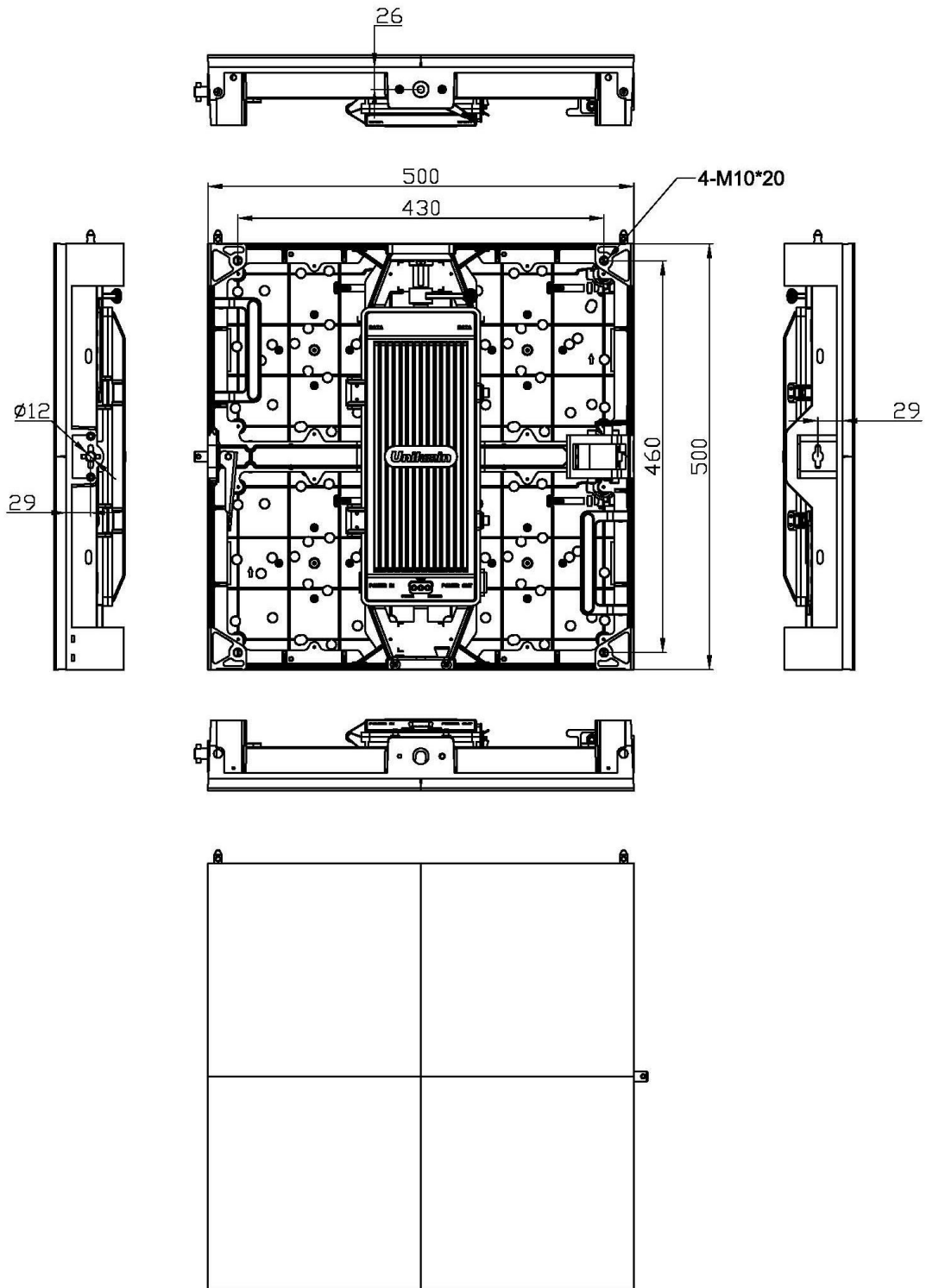
Fig1. Cabinet Dimension
