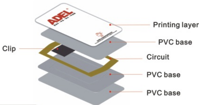
Structure of Mifare(F) hotel access card
