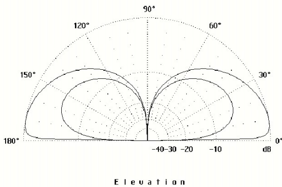
Comparison of Bravo-5 over poor ground and salt water = +12dB @ 5 degs
