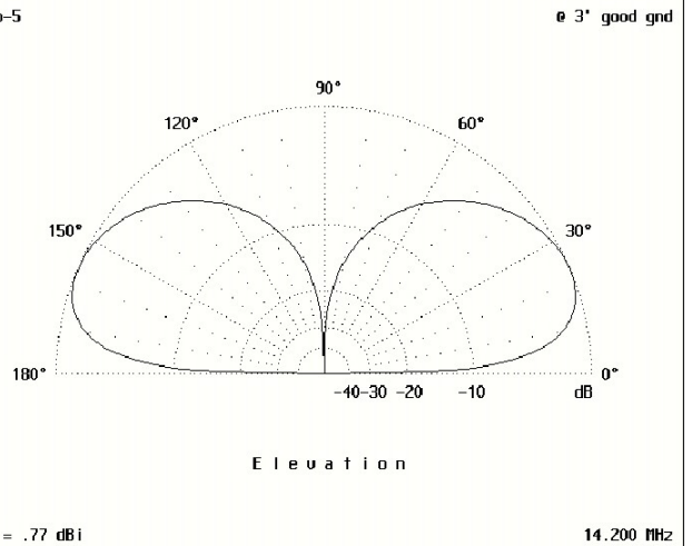
Elevation pattern for 20 meters, over ground, looking from the side.
