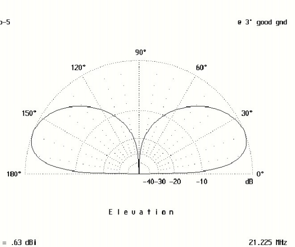
Elevation pattern for 15 meters, over ground, looking from the side.
