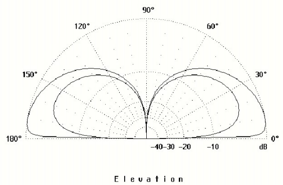
Comparison of Bravo-5 over good ground and salt water = +8dB at 5 degs
