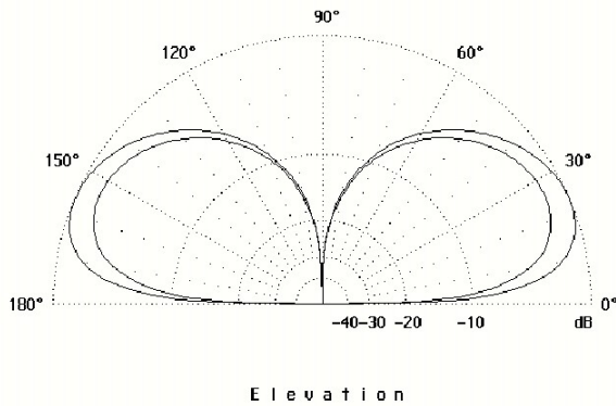
Elevation comparison of Bravo-5 over poor ground and good ground = +3dB
