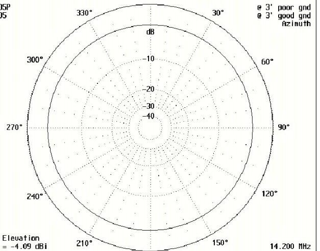
Azimuth comparison of Bravo-5 over poor ground and good ground = +3dB
